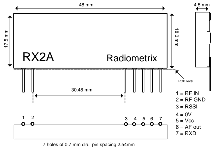
Figure 1: Physical dimensions
